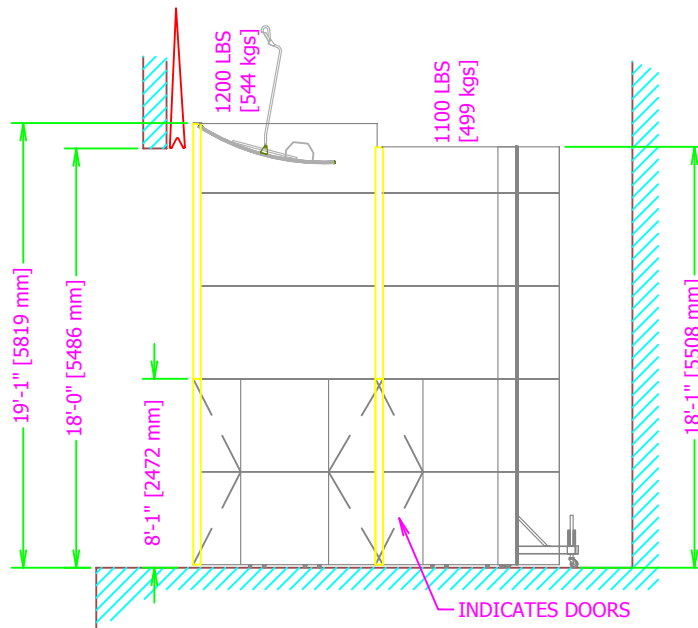
SECTION THRU CENTERLINE
