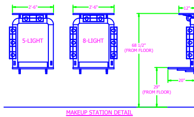
MAKEUP STATION DETAIL
