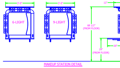
MAKEUP STATION DETAIL
