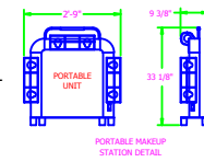
PORTABLE MAKEUP STATION DETAIL
